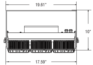
Standard Bracket / 6&8 Modules
