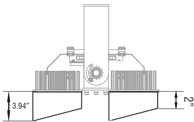
Glare Shield Visor
