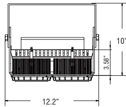
Standard Bracket / 4 Modules
