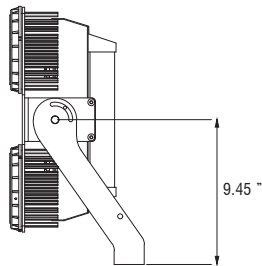
Floodlight Bracket / 4&6 Modules
