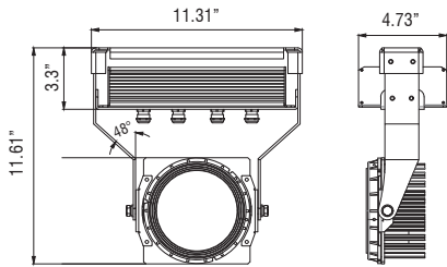
Standard Bracket / 1 Modules
