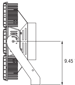
Floodlight Bracket / 8 Modules
